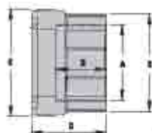
Union adaptor solvent socket
