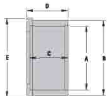
Union coupling, solvent socket outlet "BS"
